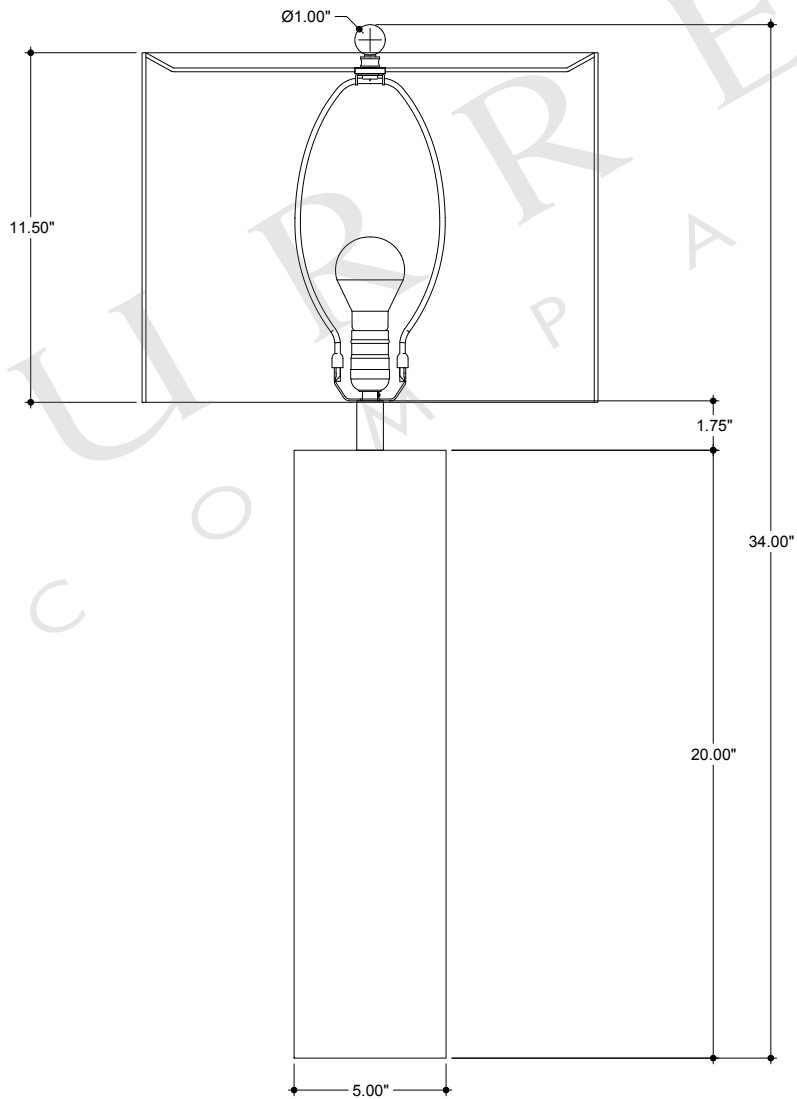
FRONT VIEW
