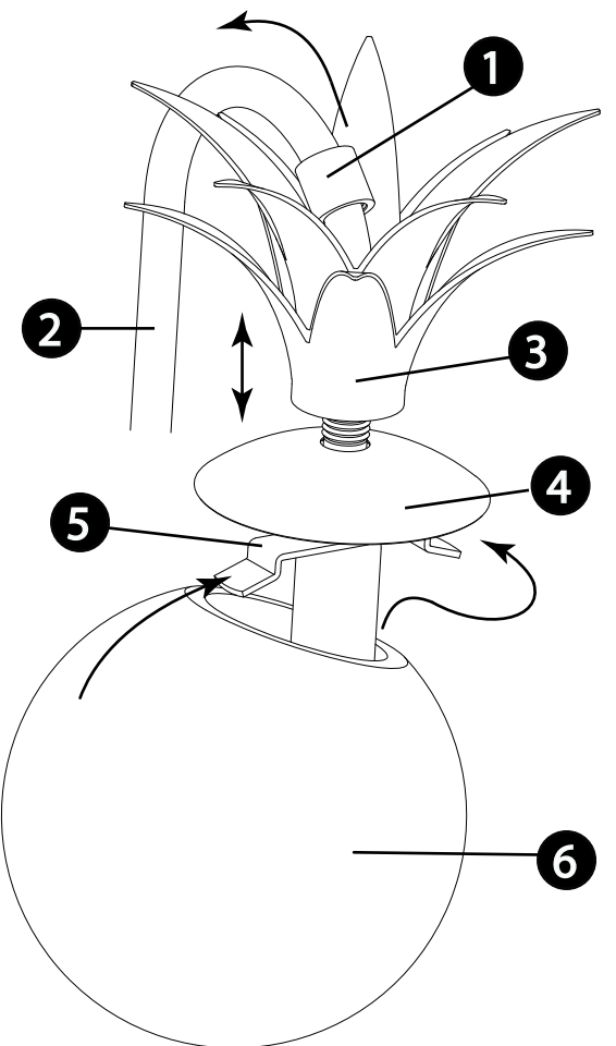
DRAWING 2 - GLASS INSTALLATION
